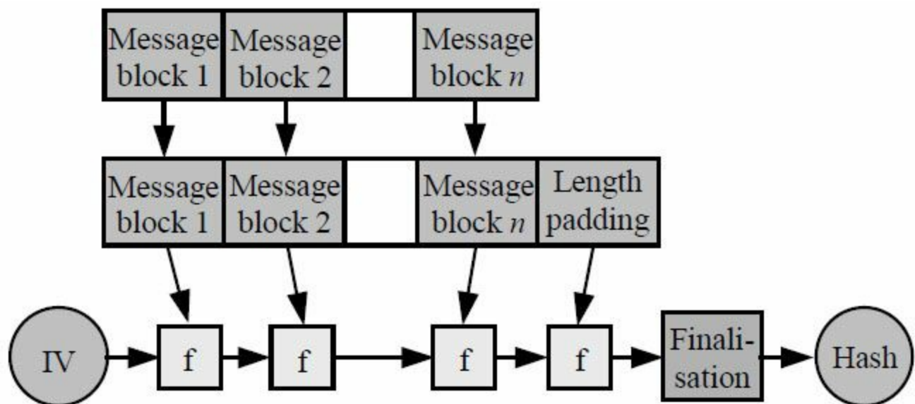
Merkle-Damgård hash construction(copied from Wikipedia)
